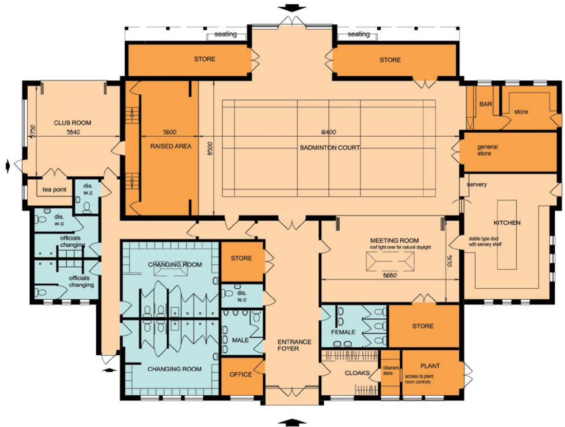
1:100 Proposed Floor Plan
